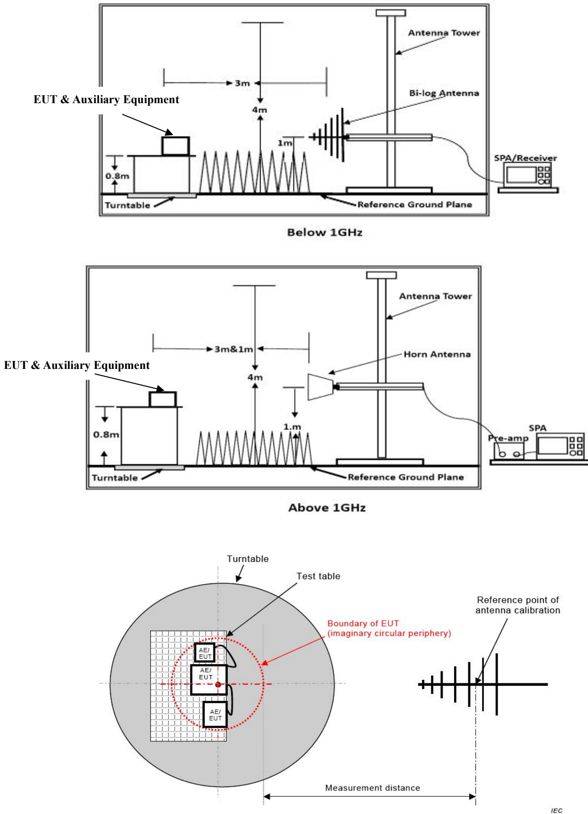
Figure C.1 – Measurement distance
