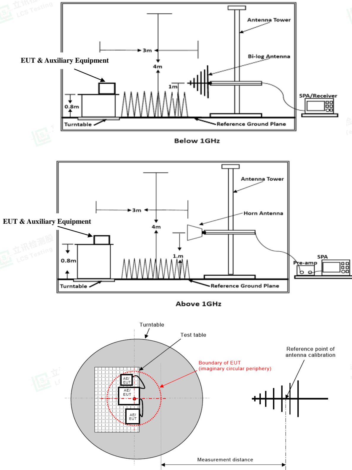
Figure C.1 – Measurement distance
