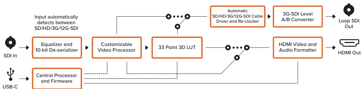
Micro Converter SDI to HDMI 12G原理图
